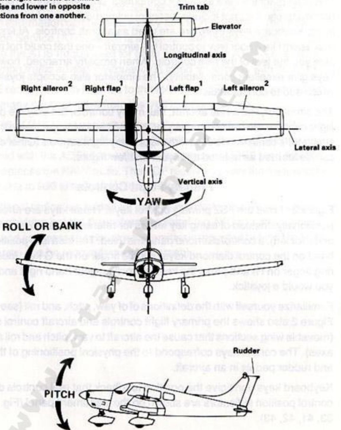
a) Control surfaces and rotational axes
