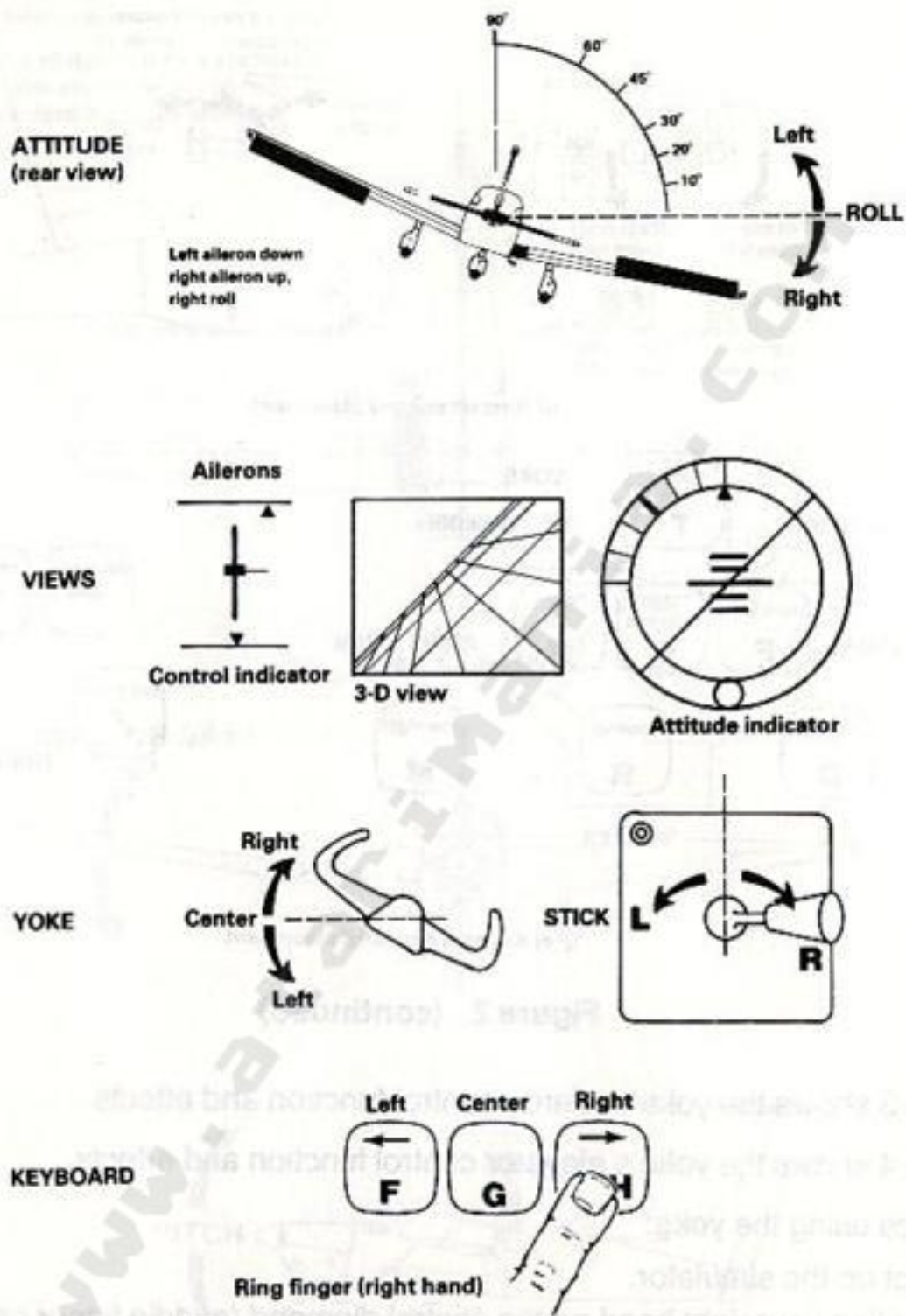
Figure 3. Ailerons – Controls and Effects
