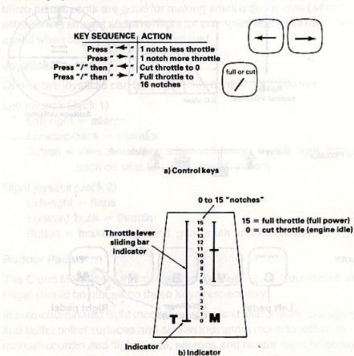
Figure 6. Throttle—Controls and Indicator
